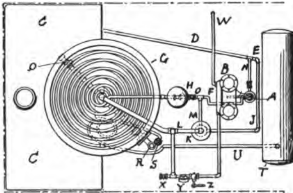
FIGS. 197-198.—Diagrams of the Fuel and Water Feed System of the White Steam Carriage. A is the water pump operated from the cross-head of the engine, B. C is the water tank; D, a pipe leading to the pump, and branching off at E, as shown, into J and N. F is the boiler feed pipe leading through the check valve, O, and the air chamber, H. K is the automatic by-pass regulator; L, a pipe leading steam from the generator, G, and allowing the water to circulate through F M K J E N A, whenever steam pressure rises high. X, the pop valve; Y, the gauge; Z, the throttle; T, the fuel tank; U, the fuel feed pipe; Q R S, the fuel regulating and vaporizing system explained later.
